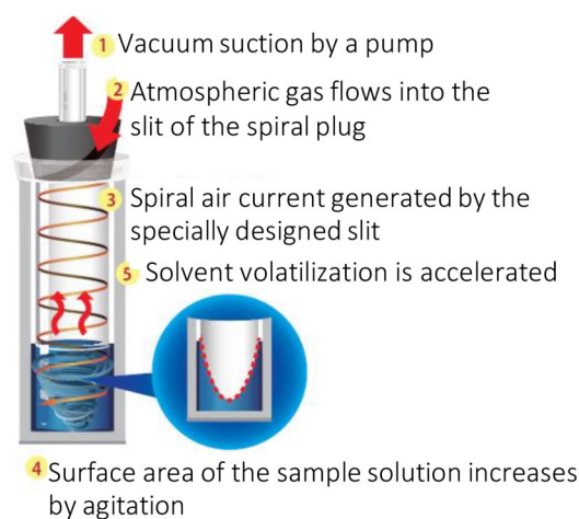
Fig. 2 Mechanism of VVCmethod
